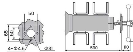
Operation outside 2000~2500A board
