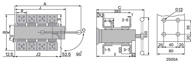
Direct operation on front face of 3150A
