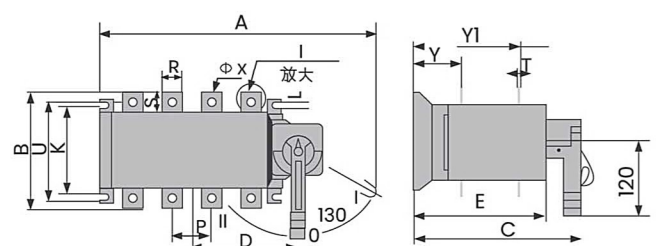
Direct operation of 100~1600A
