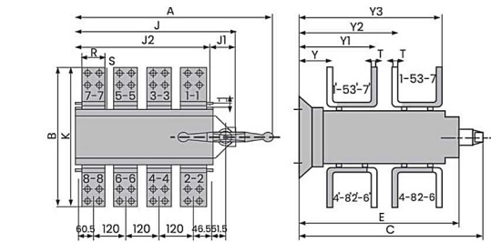
Direct operation in front face of 2000~2500A
