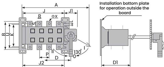
Operation outside 100~1600A board
